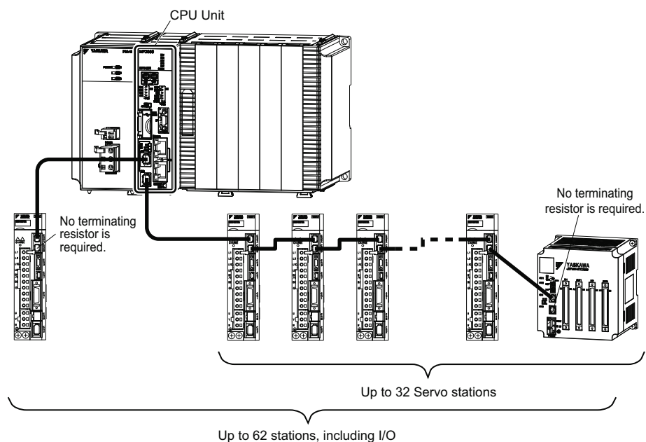
Figure 2 Cascaded Connections Using Two Ports
